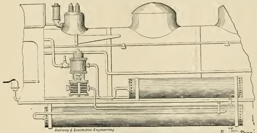
Fig. 2.—PROPOSED COOLING PIPE AND MAIN RESERVOIR LOCATION.
